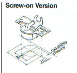
(Old) 830 Hinge Layout
